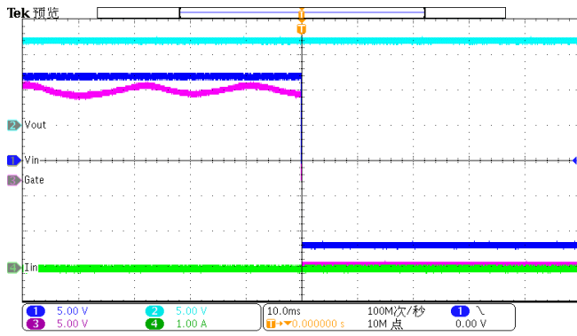
Figure 16. Static Reverse Polarity
